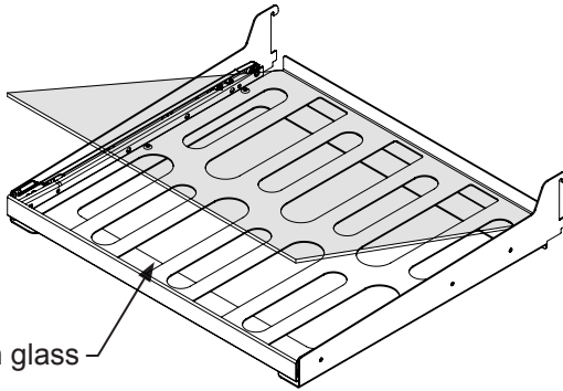
Figure 31 Wine cutout and flat glass shelf with vibration dampening mat, the glass can be removed for wine storage.
