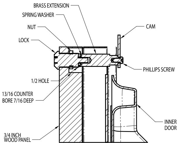
SECTION A-A SCALE 1:1 Figure 23
